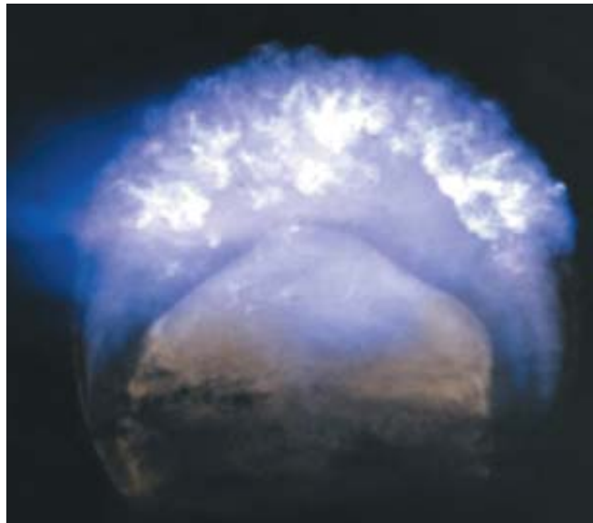
ORANGE WAS THE CODE NAME for a 1958 burst of a 3.8-megaton nuclear device at an altitude of 43 kilometers. The test had little effect on radio communications and electrical systems in the Pacific area.
